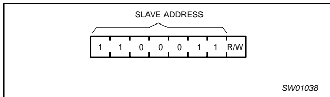
Figure 4. Slave address — PCA9553/02
