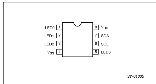
Figure 1. Pin configuration
